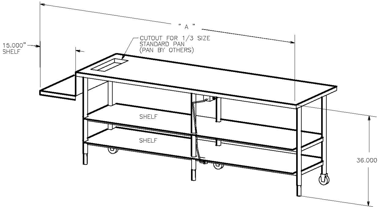
Overall Dimensions Heated Sandwich Wrap Table
